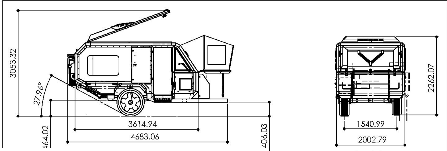
Front view (Closed)
