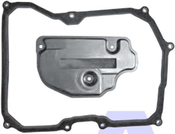
AISIN WARNER TF-60SN (09G) Pan Gasket 09G.GAS01 Filter 09G.FIL01 No Pick Up
