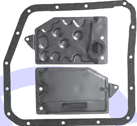
AISIN WARNER A140E Pan Gasket A130.GAS01 Filter A140.FIL01
