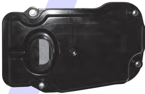
AISIN WARNER AB60E/F 6 SPEED TOYOTA Pan Gasket AB60E.GAS51 Filter AB60E.FIL01
