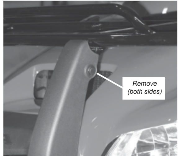
Figure 1 Remove the Two Plastic Rivets
