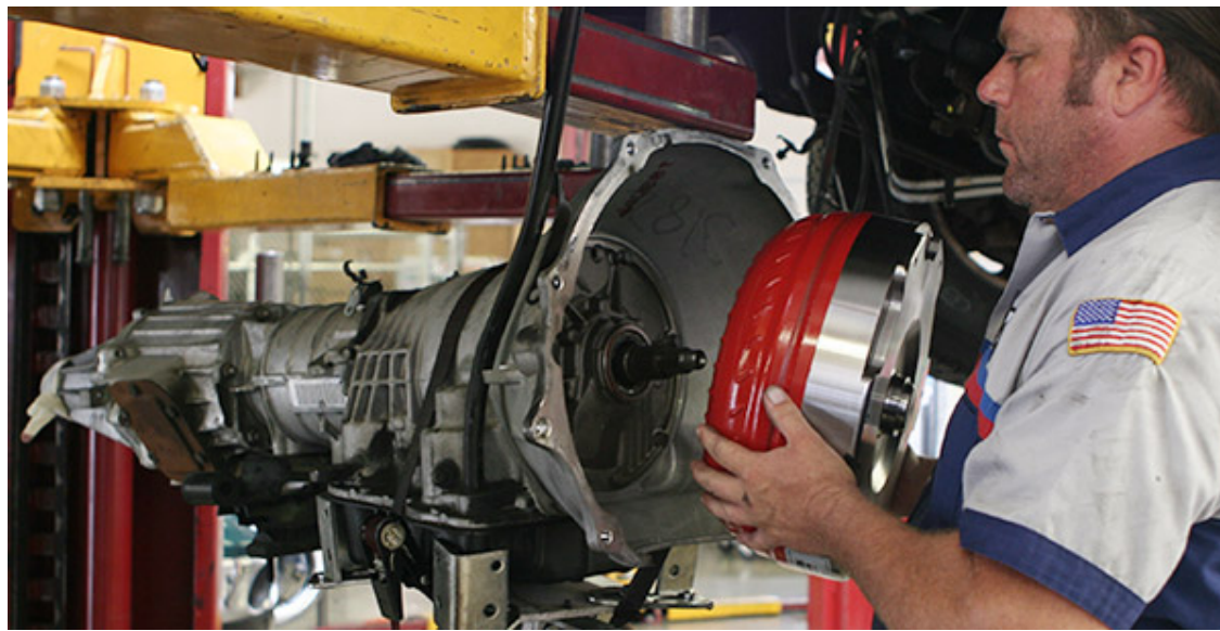
Banks Billet Torque Converter installation.
