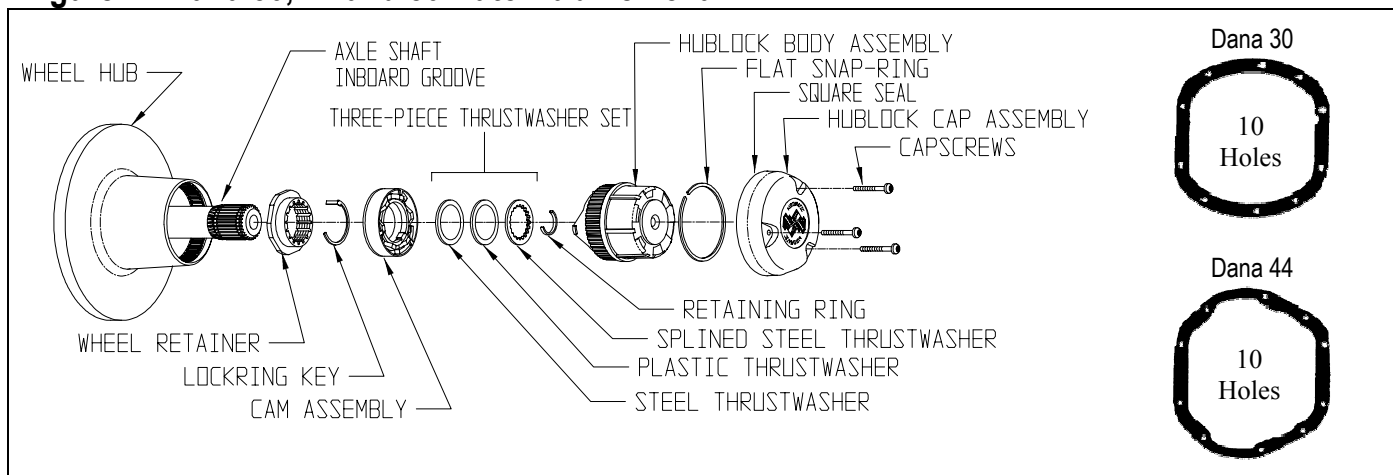
Figure 1: Dana 30, 44 and 50 Auto Hub Removal
