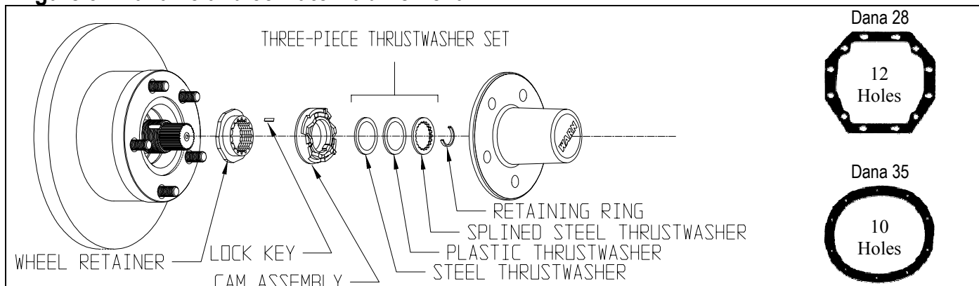
Figure 3: Dana 28 and 35 Auto Hub Removal
