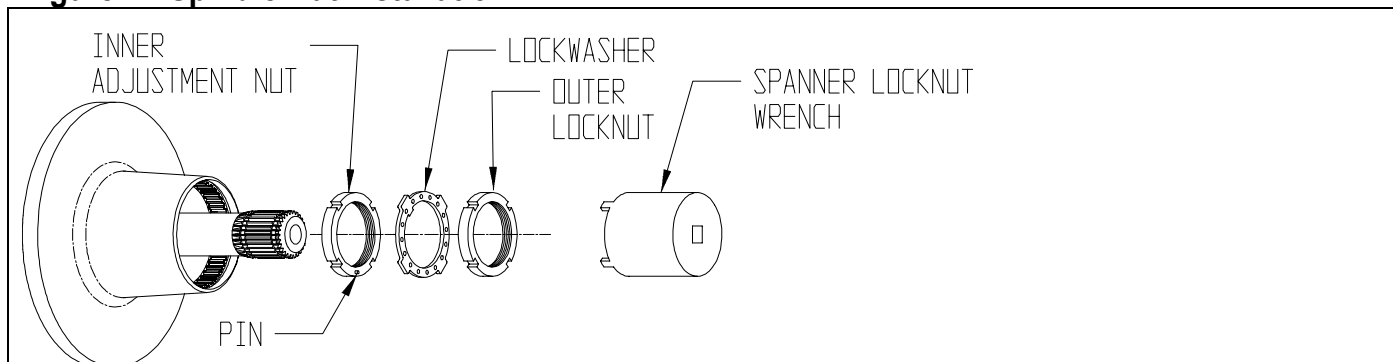
Figure 4: Spindle Nut Installation
