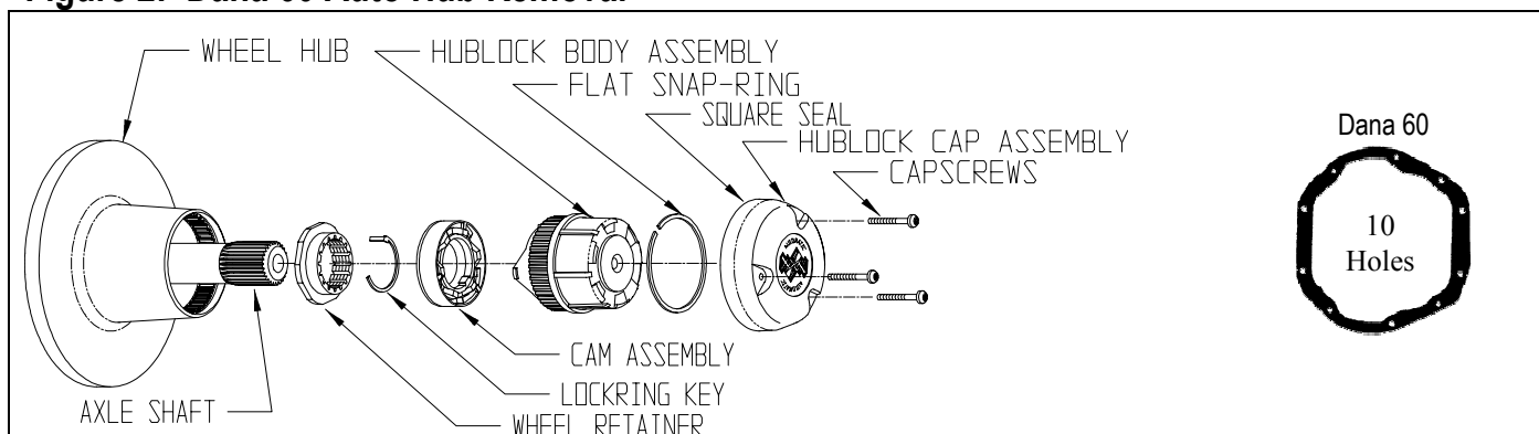
Figure 2: Dana 60 Auto Hub Removal
