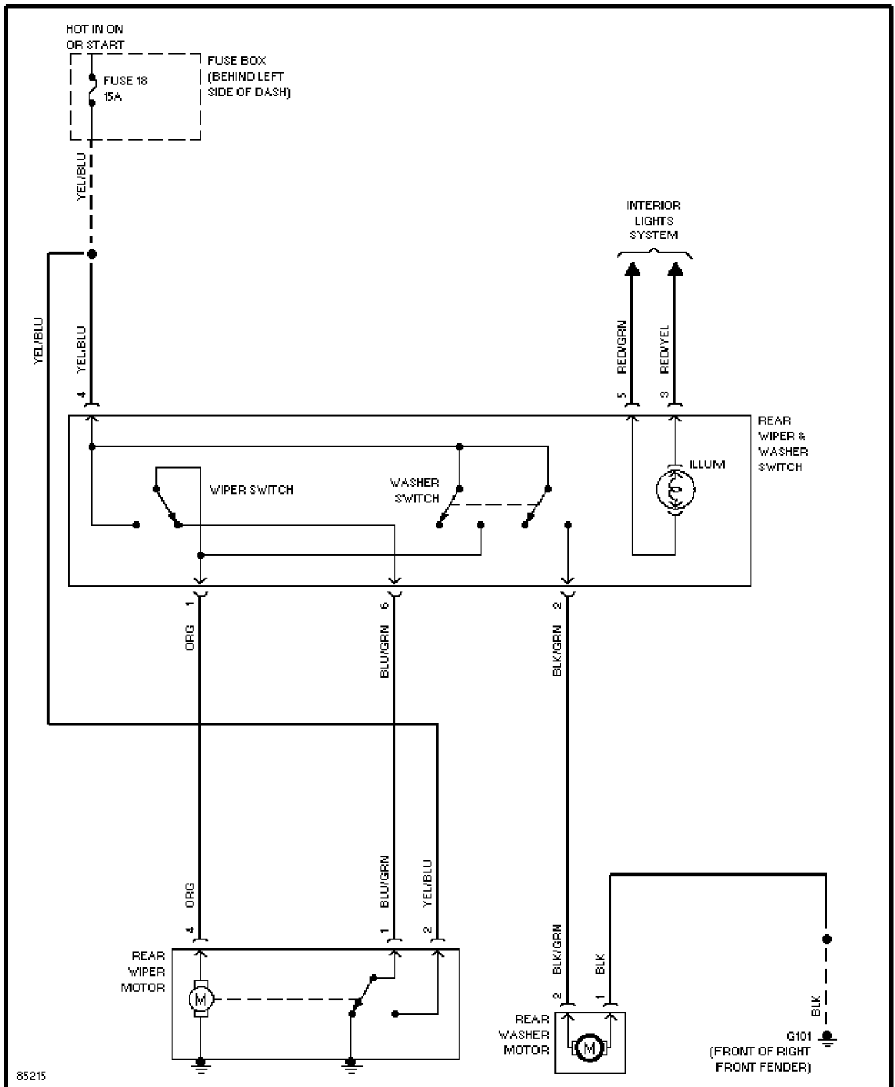
1.6L, Rear Wiper/Washer Circuit
