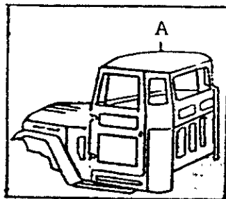
FIG. 08/05 - CABINE P/ PICK-UPS E COMPONENTES
